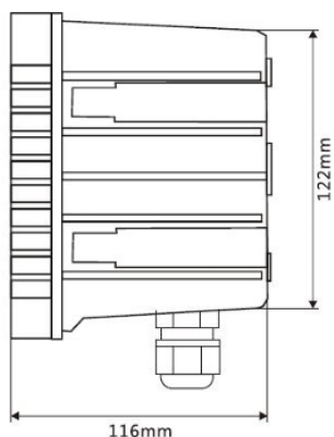
144 series dimension
